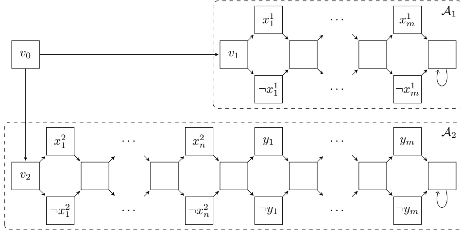
■ Figure 10 The single-player arena \mathcal{A} used in the reduction from the \Sigma_2\text{QBF}^{\text{neg}} problem.
