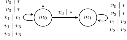
■ Figure 5 A nondeterministic Mealy machine of player 0. The notation v | v' on the transitions (m, m') indicates that m' \in \delta(m, v) , and if v \in V_0 , that v' \in \tau(m, v) , otherwise v' = * .
