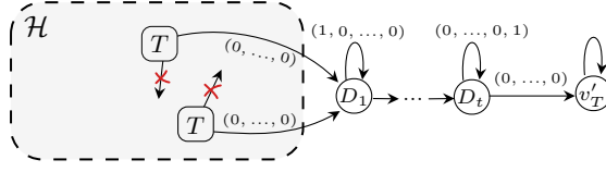
■ Figure 7 Reduction from the SP problem to the ESP problem.
