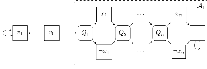
■ Figure 11 The arena used in the reduction from coQBF.
