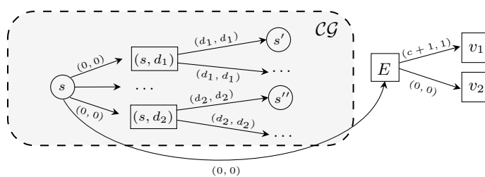
■ Figure 15 Reduction from countdown games to the NCNS problem with two players and bounded reachability objectives.
