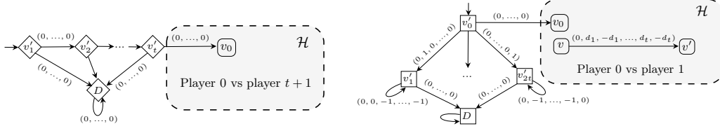
■ Figure 8 Reduction from the SP problem to the NCNS problem. ■ Figure 9 Reduction from the ESP problem to the NCNS problem.
